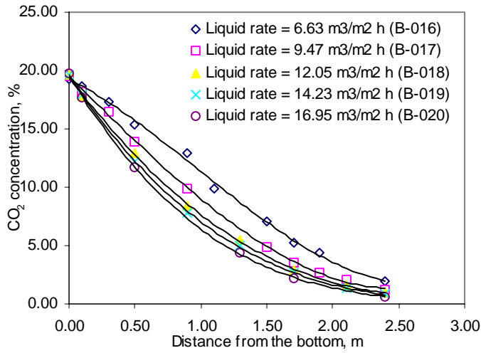
Figure 4. Effect of liquid flow rate on CO 2 absorption into MEA solutions.
