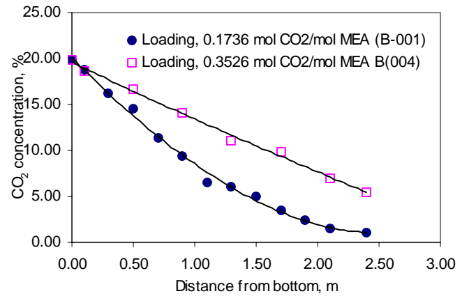
Figure 7. Effect of CO 2 loading on the absorption process
