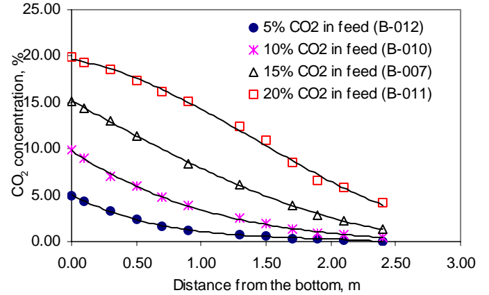
Figure 6. Effect of gas CO 2 concentration on the absorption rate.
