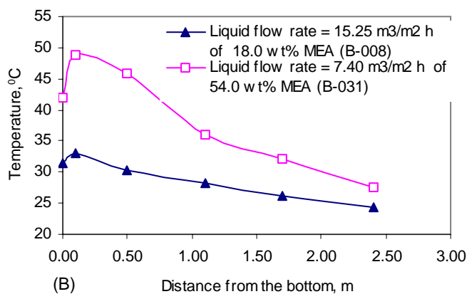
Figure 2. The effect of absorbing the same quantity of CO 2 in a smaller volume of solution on the temperature profile. Runs number: B-008 and B-031.
