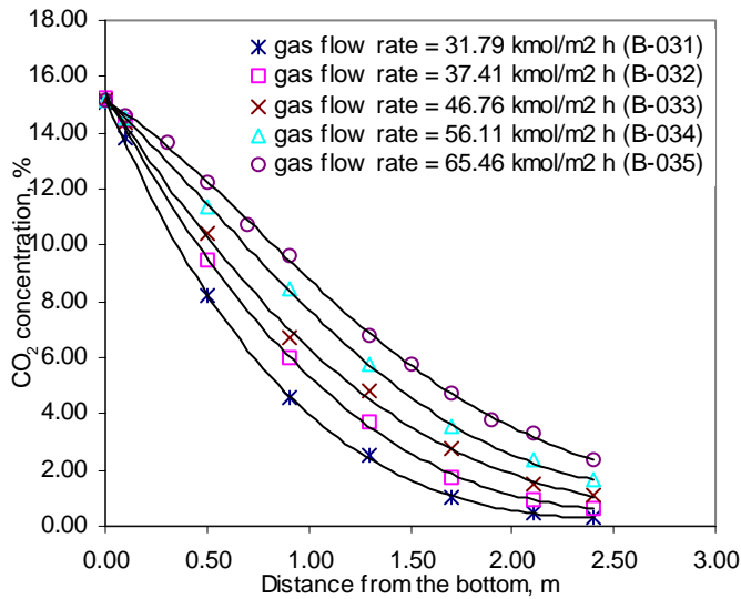
Figure 5. Effect of gas flow rate on the CO 2 absorption
